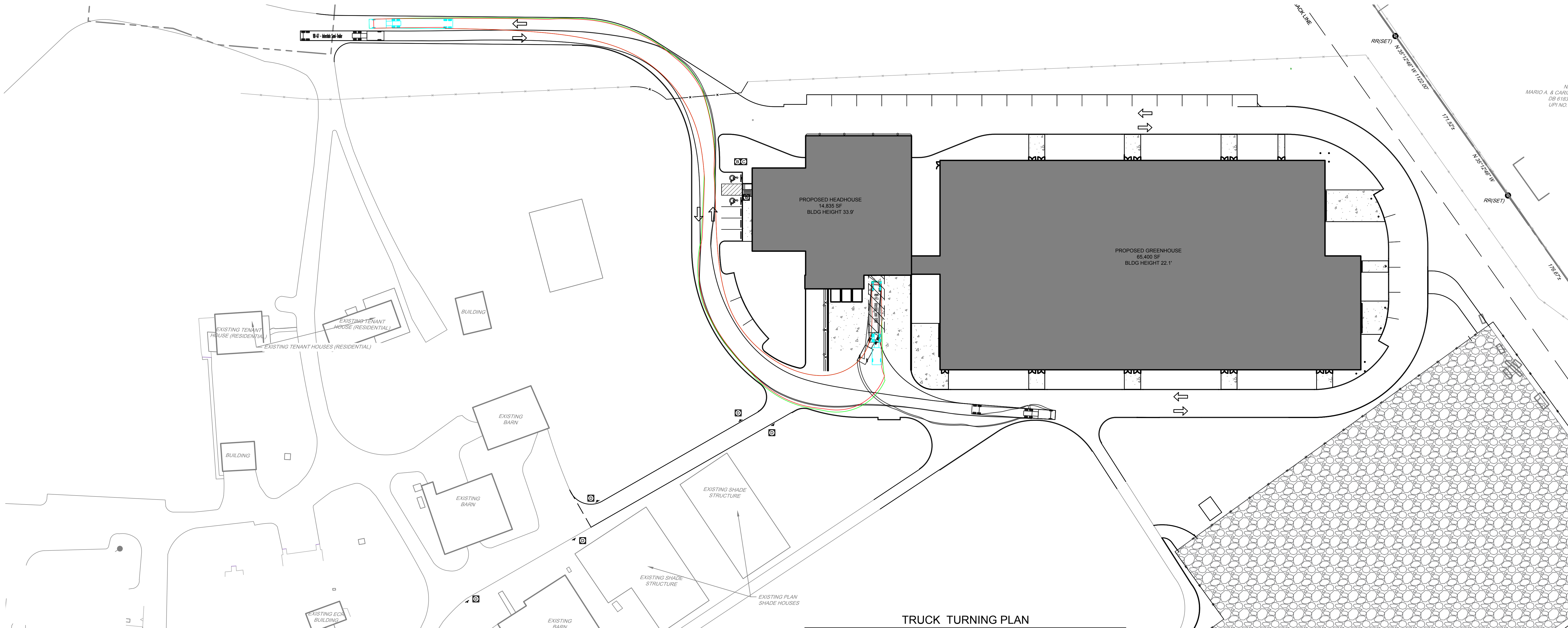
TRUCK TURNING PLAN SCALE: 1" = 40'
