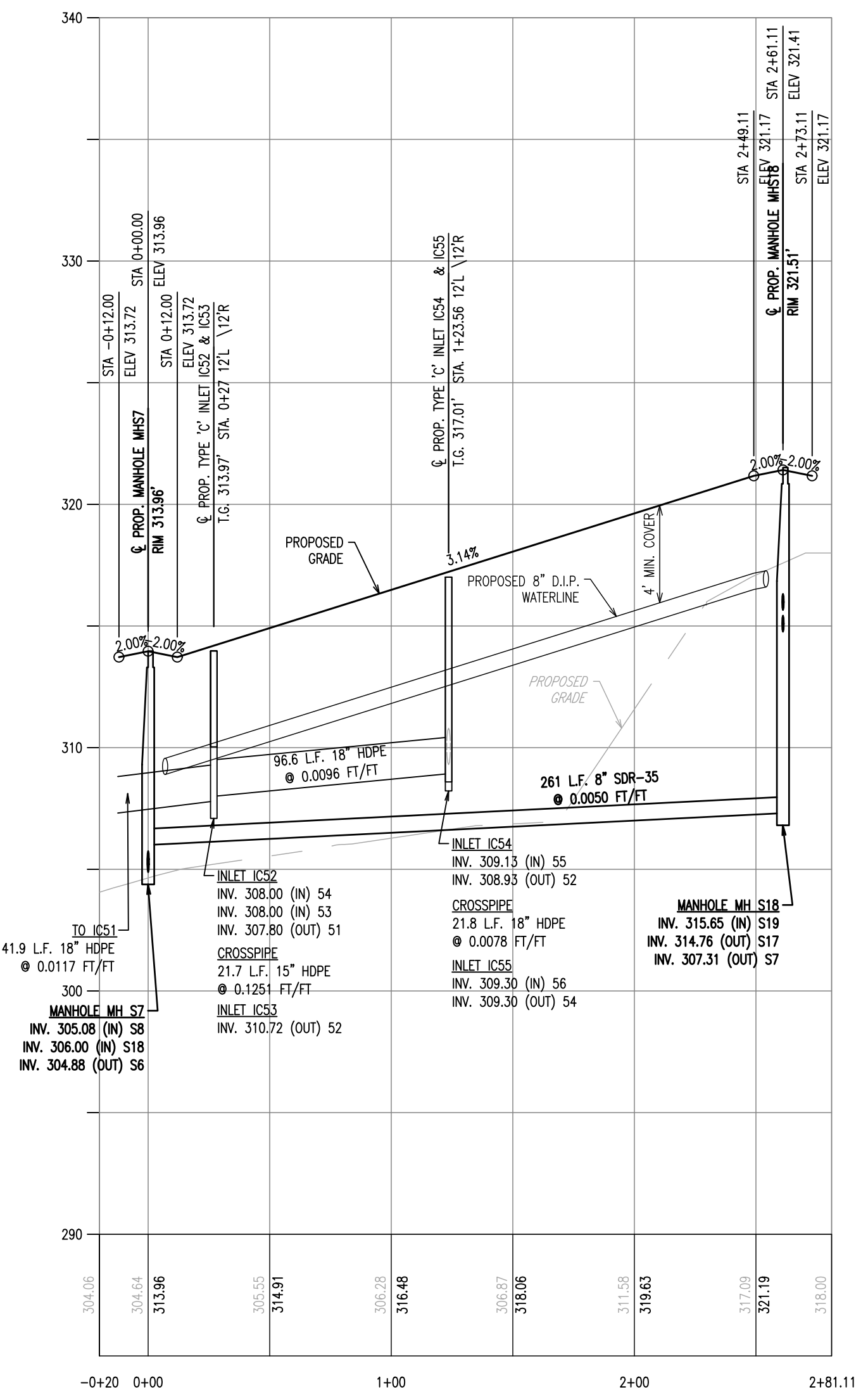
DRIVE 3 PROFILE STA -0+20 - 2+81.11
