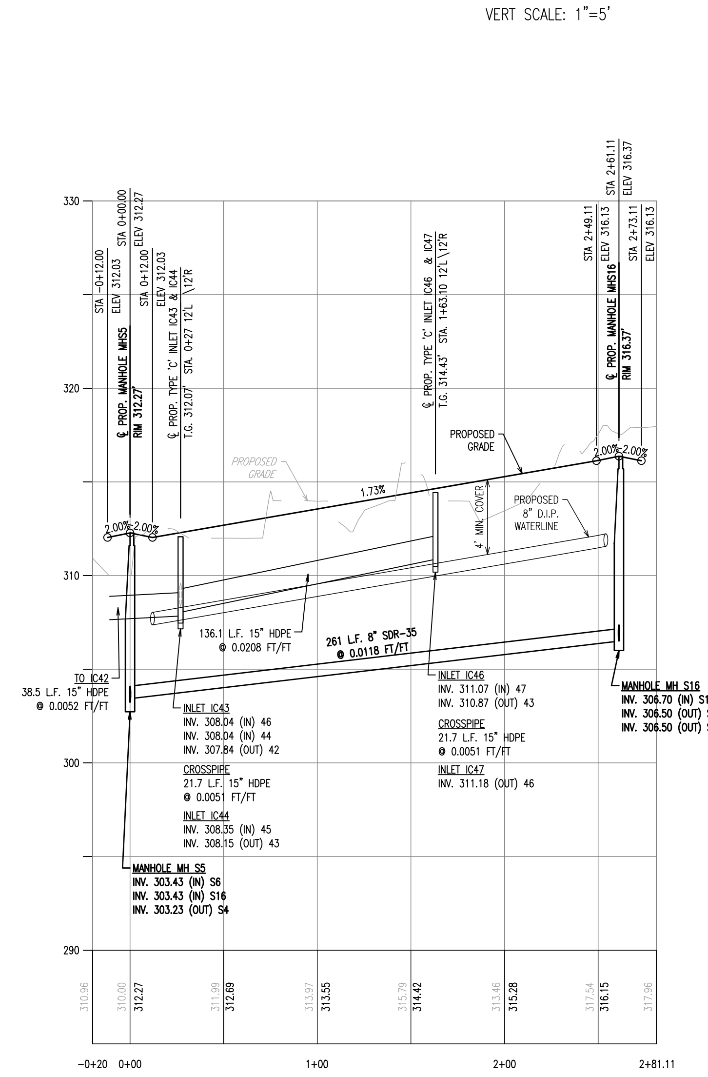
DRIVE 2 PROFILE STA -0+20 - 2+81.11
