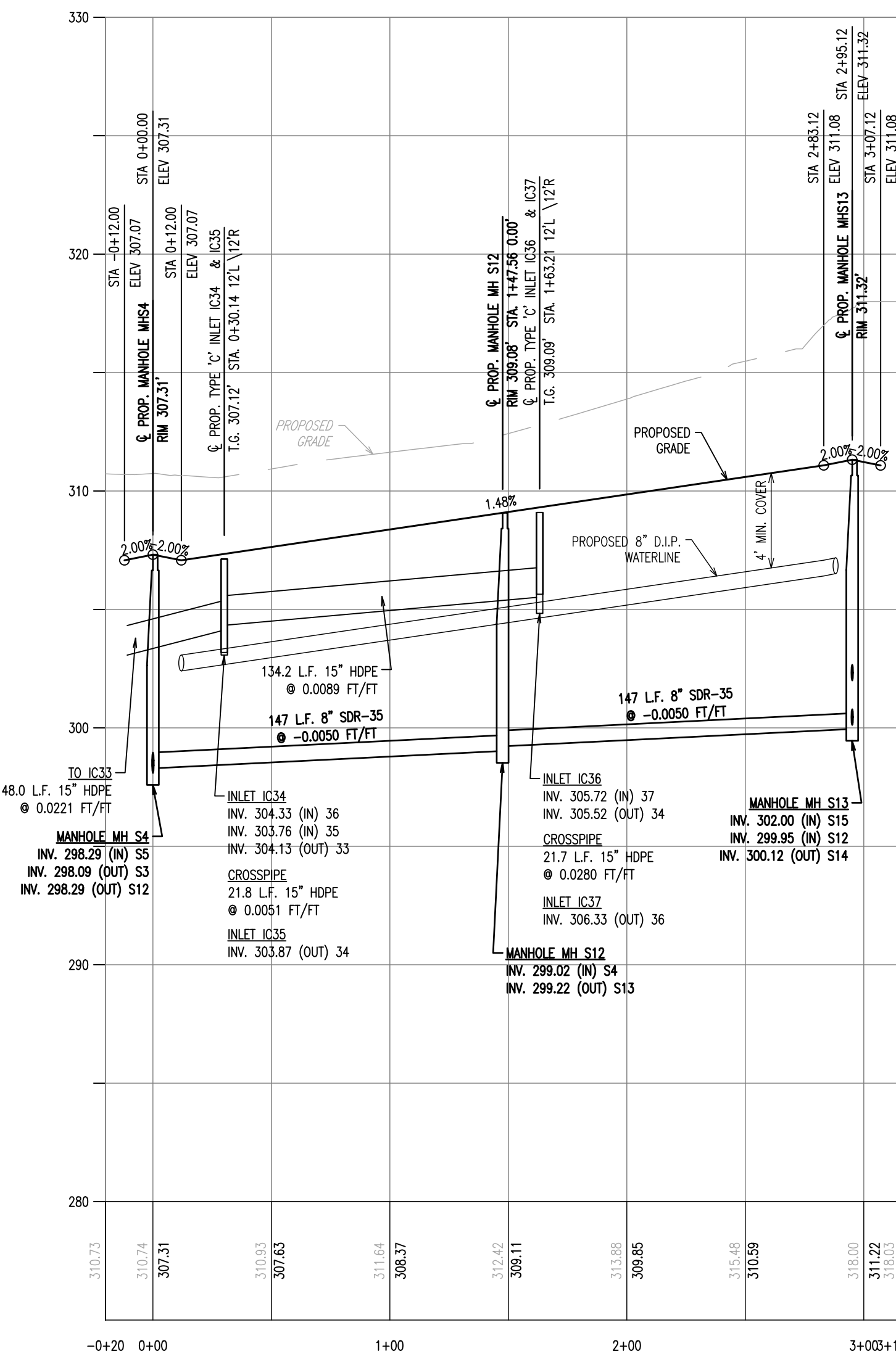
DRIVE 1 PROFILE STA -0+20 - 3+15.12
