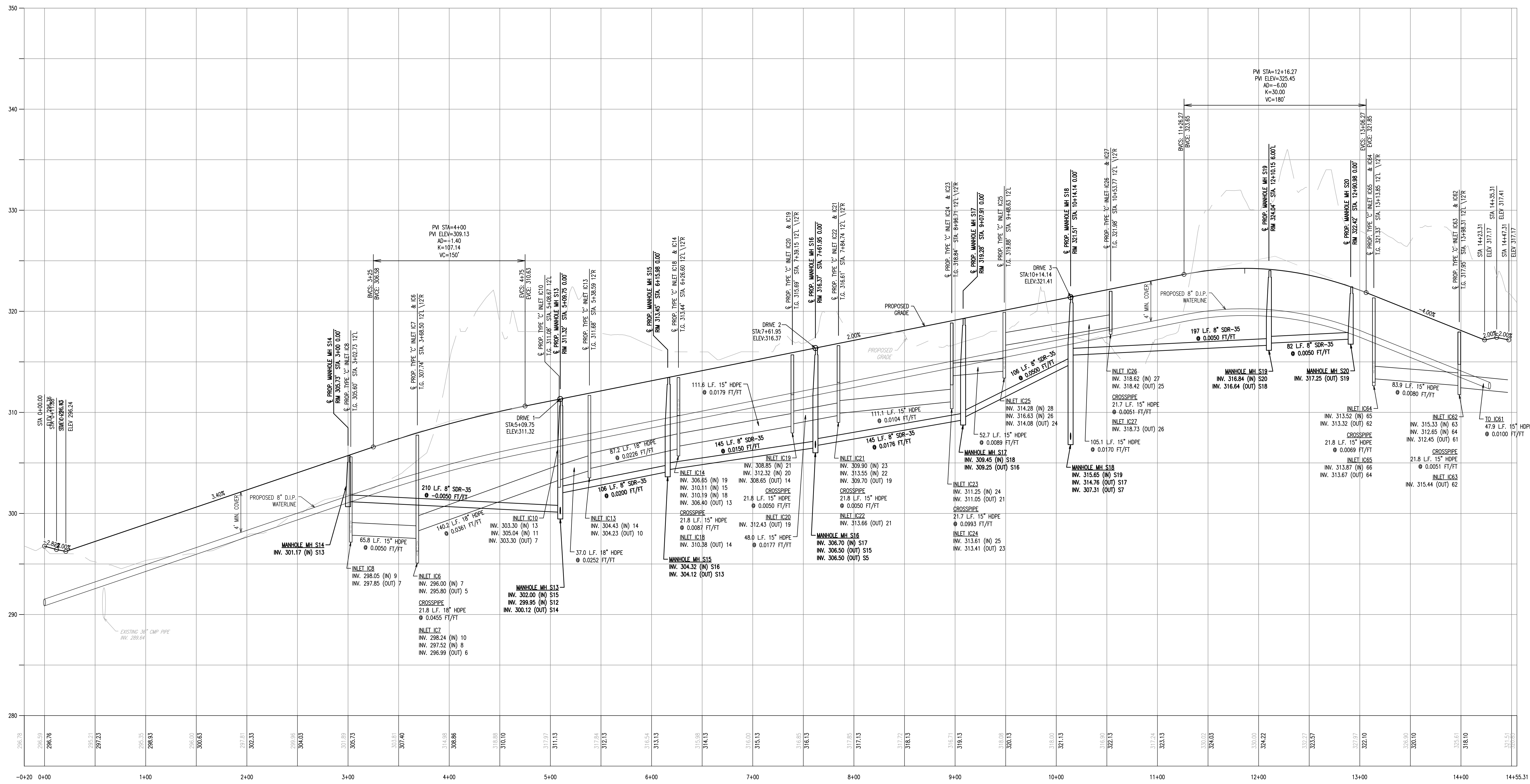
INTERNAL DRIVE B PROFILE STA -0+20 - 14+55.31
