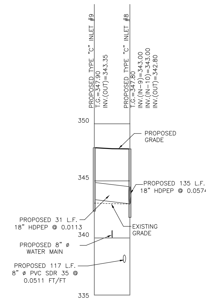
STORM SEWER PROFILE PROPOSED INLET #9 TO PROPOSED INLET #8 SCALE: HORIZ. 1"=50' VERT. 1"=5'
