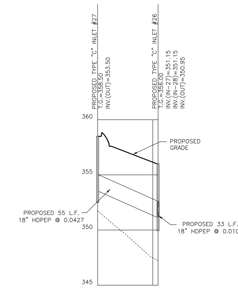
STORM SEWER PROFILE PROPOSED INLET #27 TO PROPOSED INLET #26 SCALE: HORIZ. 1"=50' VERT. 1"=5'
