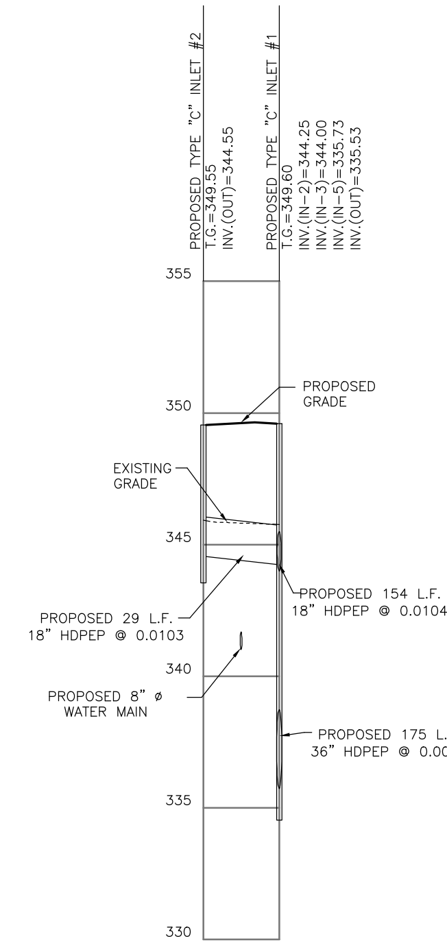
STORM SEWER PROFILE PROPOSED INLET #2 TO PROPOSED INLET #1 SCALE: HORIZ. 1"=50' VERT. 1"=5'
