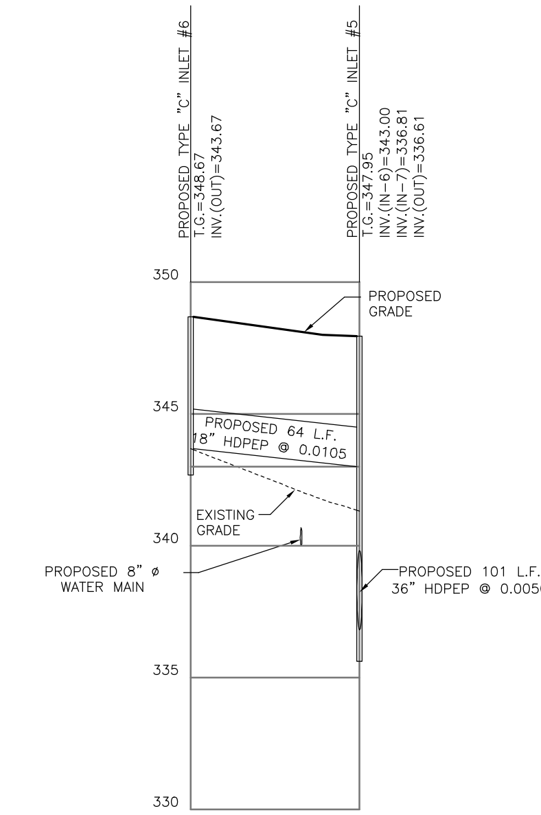
STORM SEWER PROFILE PROPOSED INLET #6 TO PROPOSED INLET #5 SCALE: HORIZ. 1"=50' VERT. 1"=5'
