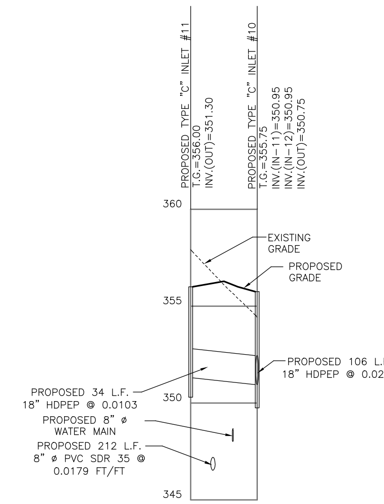
STORM SEWER PROFILE PROPOSED INLET #11 TO PROPOSED INLET #10 SCALE: HORIZ. 1"=50' VERT. 1"=5'
