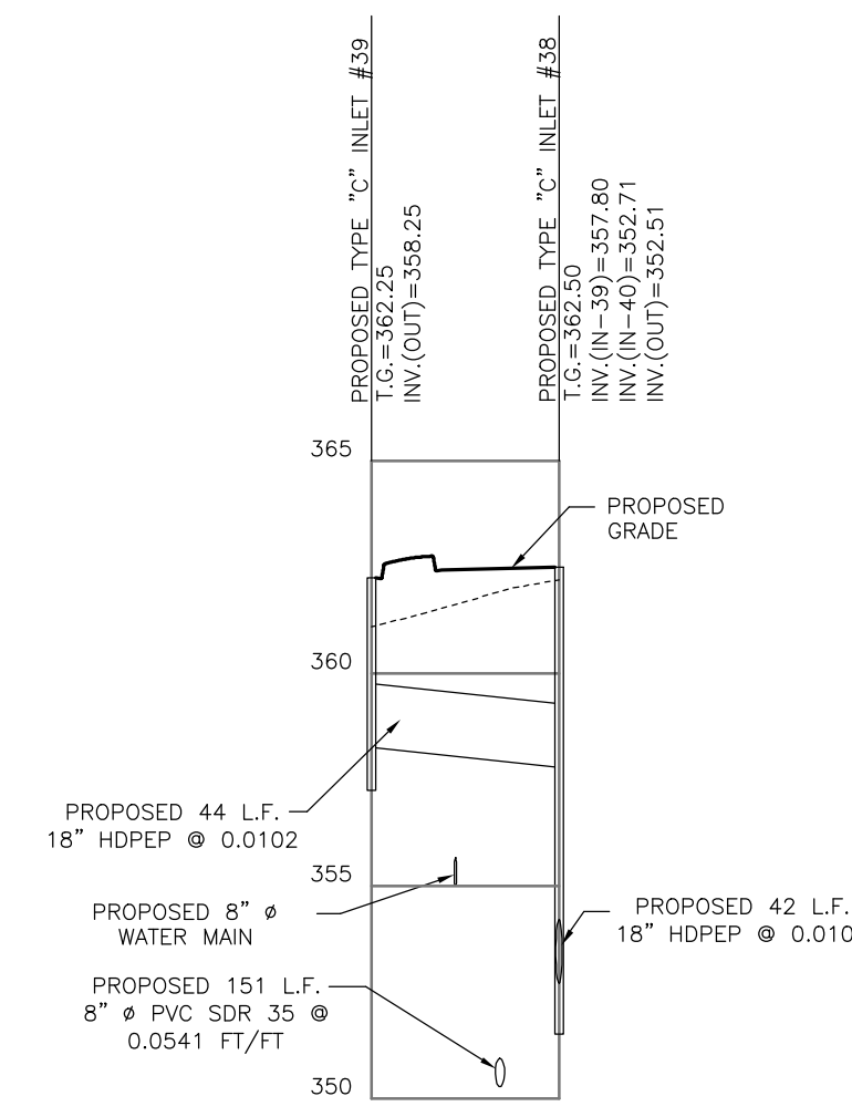
STORM SEWER PROFILE PROPOSED INLET #39 TO PROPOSED INLET #38 SCALE: HORIZ. 1"=50' VERT. 1"=5'
