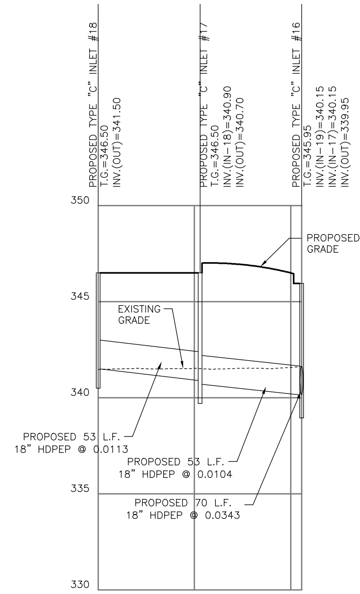
STORM SEWER PROFILE PROPOSED INLET #18 TO PROPOSED INLET #16 SCALE: HORIZ. 1"=50' VERT. 1"=5'
