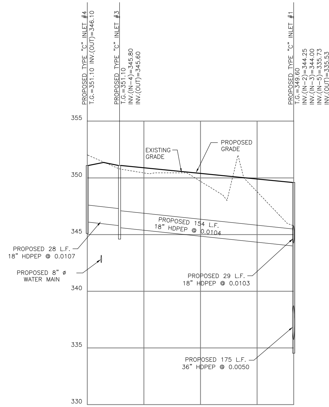
STORM SEWER PROFILE PROPOSED INLET #4 TO PROPOSED INLET #1 SCALE: HORIZ. 1"=50' VERT. 1"=5'
