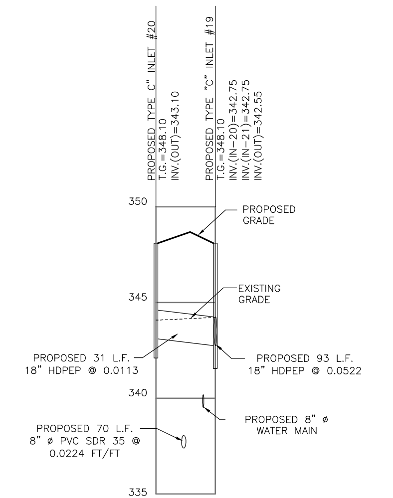
STORM SEWER PROFILE PROPOSED INLET #20 TO PROPOSED INLET #19 SCALE: HORIZ. 1"=50' VERT. 1"=5'
